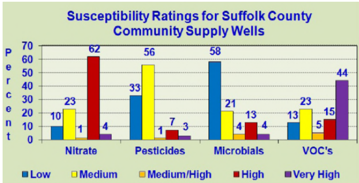
Figure 5.4.9-7. Susceptibility Ratings for Suffolk County Community Supply Wells
