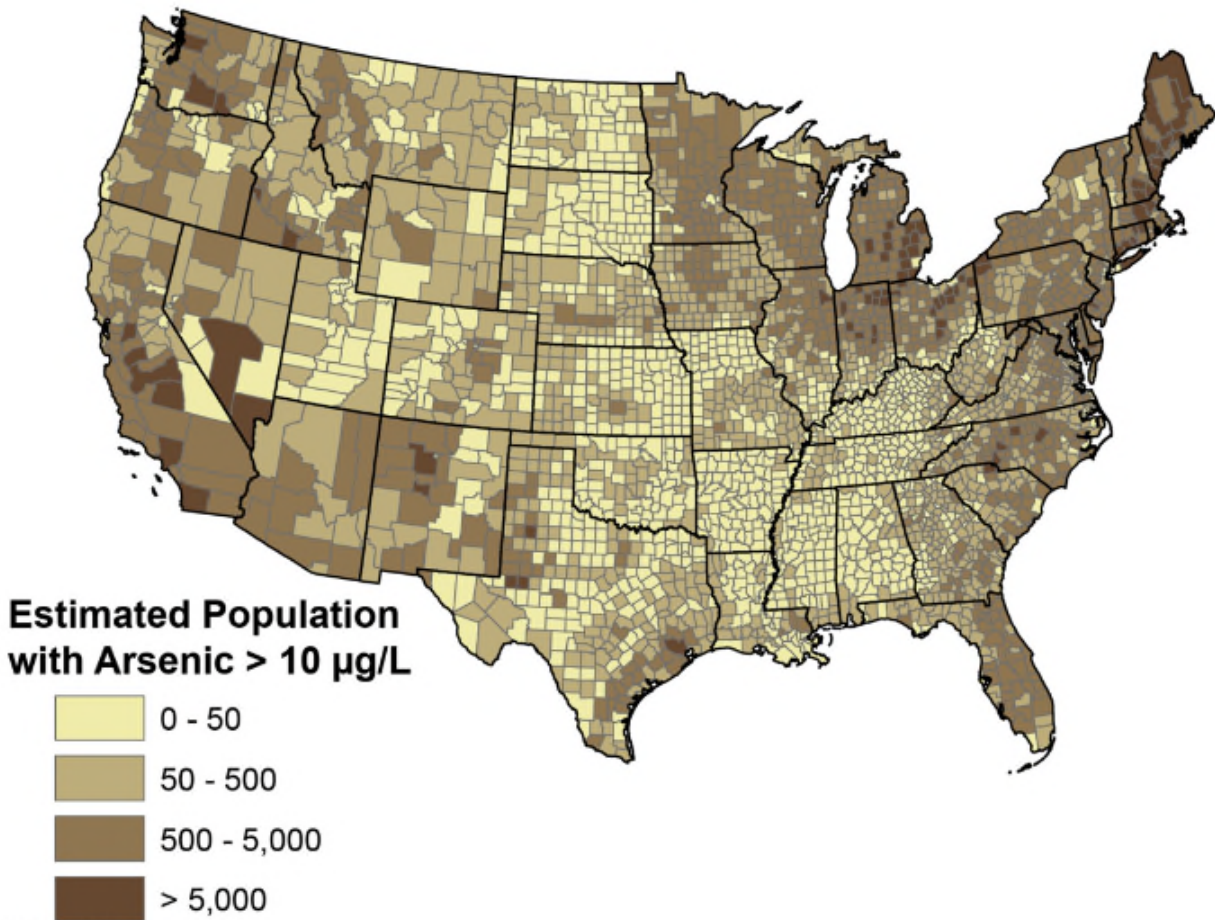
Figure 5.4.9-5. Estimated Population with Arsenic >10 Micrograms Per Liter
