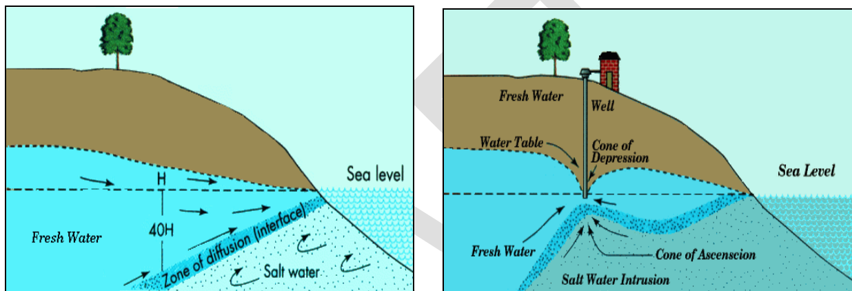
Figure 5.4.9-1. Saltwater Intrusion Process
