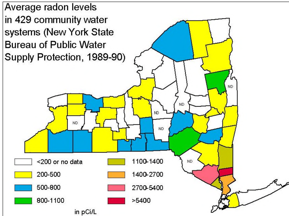
Figure 5.4.9-3. Average Radon Levels of 429 Community Water Systems (1989-1990)
