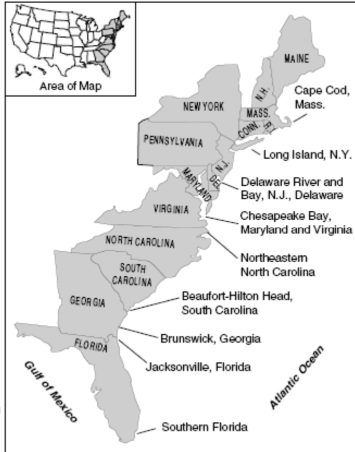
Figure 5.4.9-6. Selected areas along the Atlantic coast where saltwater has intruded into freshwater aquifers.
